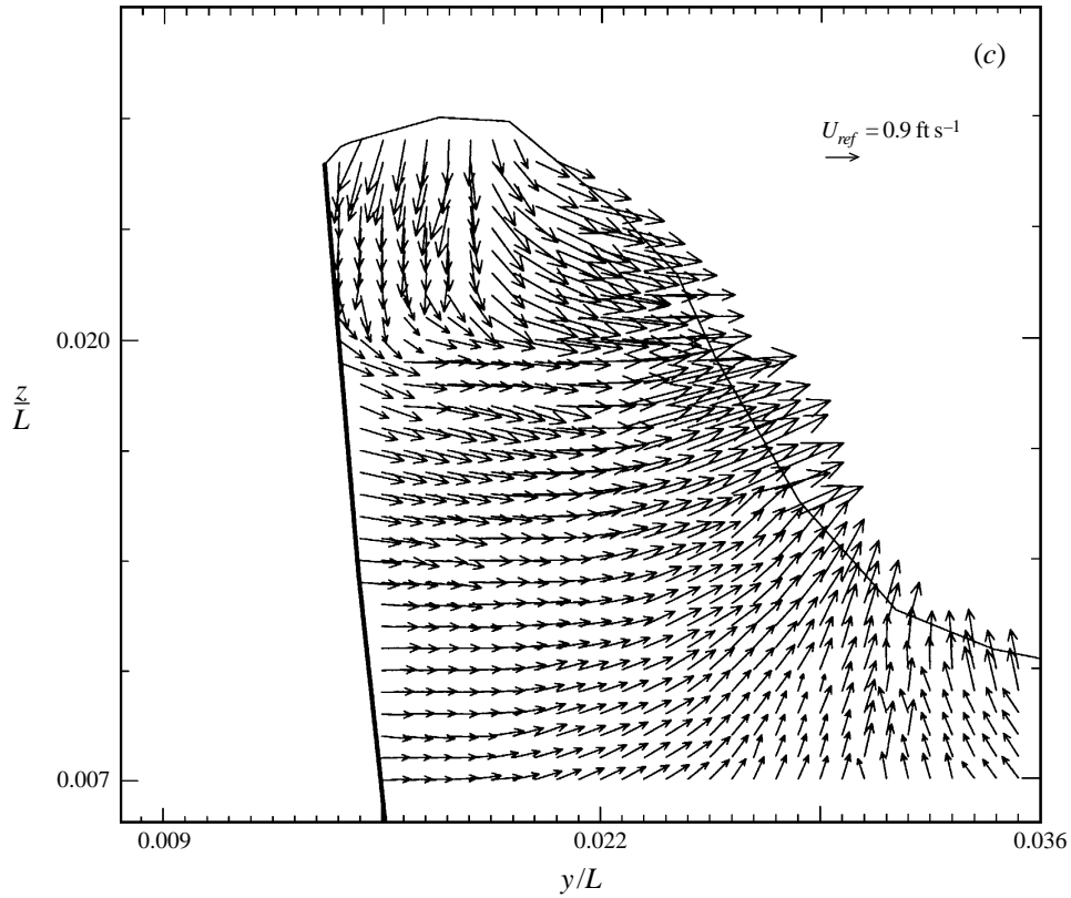
FIGURE 14. (a) Velocity and (b) vorticity ( \omega L/U ) distributions at X/L = 0.08 and Fr_L = 0.446 . (c) Magnified portion of the velocity field after subtracting a constant reference velocity (identified as U_{ref} ).
