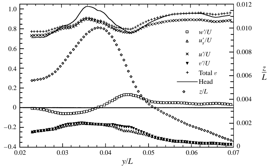
FIGURE 18. Distributions of all three components of the velocity, the total speed and the total head along the free surface at X/L = 0.10 and Fr_L = 0.279 . The data are presented in the ship frame of reference and the corresponding coordinates (x', y', z') are defined in figure 1(b). The velocity is determined using the experimental data and by assuming that u_n = 0 .
